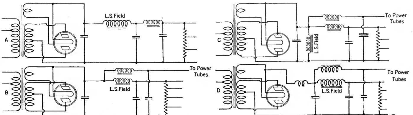
Fig. 1—These diagrams illustrate four methods which may be used for obtaining all potentials required for the operation of a receiver without exceeding the rating of a standard UX-245 full-wave rectifier tube. Each of these power supply systems is designed to supply a receiver of different voltage and current requirements.
