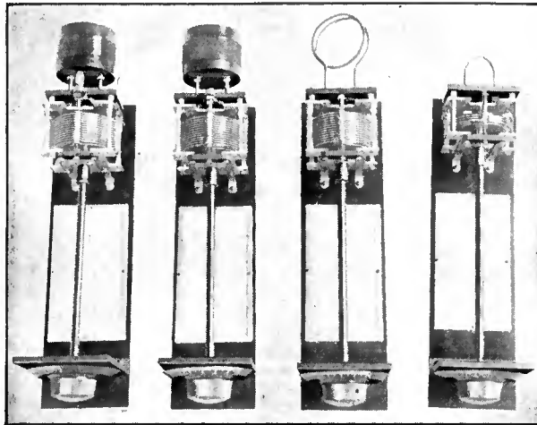
Fig. 1—Knockabout wavemeters are used at the Radio Frequency Laboratories for preliminary adjustments. This picture shows four such instruments of different wavelength ranges.
