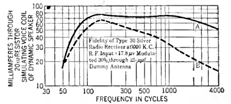
Fig. 4—(A) Overall fidelity curve of the receiver. (B) How the fidelity may be changed with the "overtone cut-out switch."
